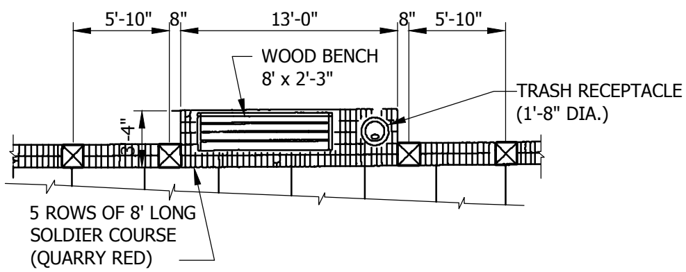
BENCH AREA DETAIL
